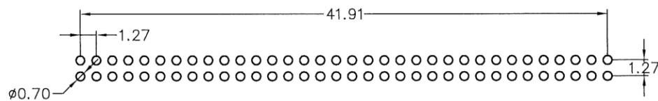
RECOMMENDED PCB LAYOUT (PCB TOLERANCE:±0.05)
